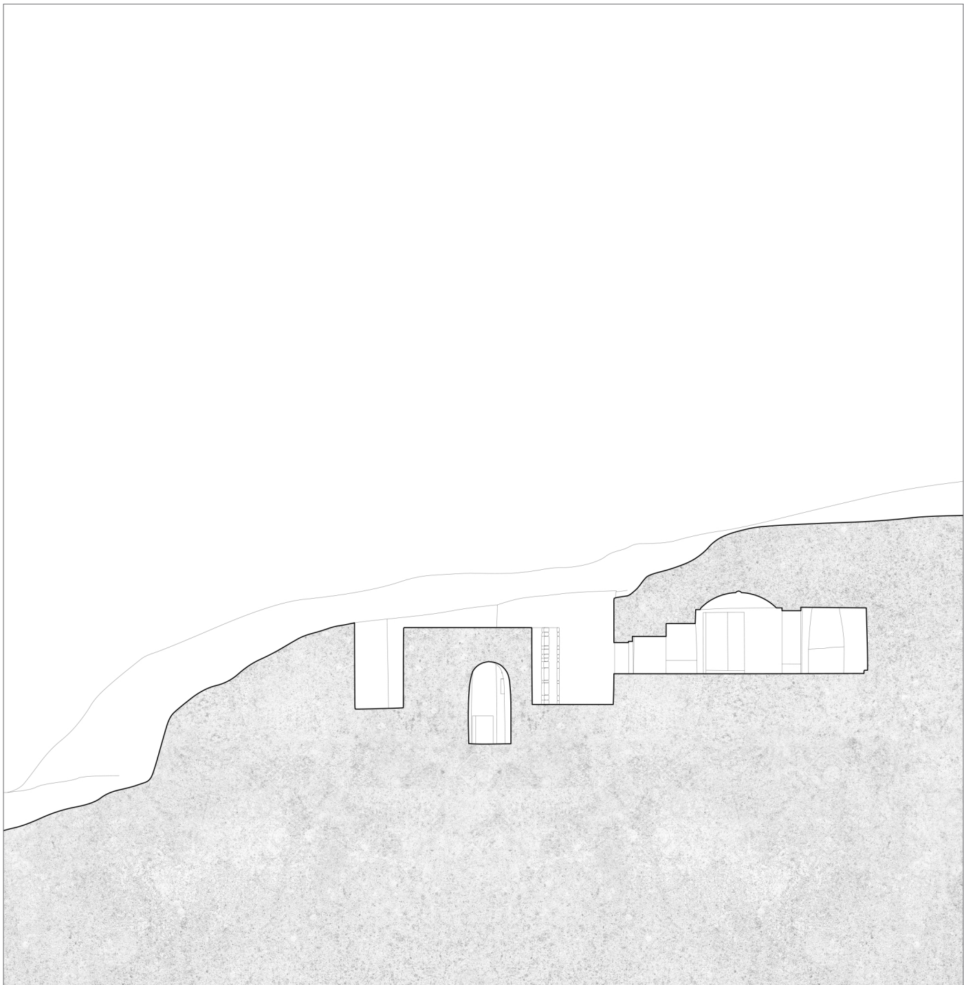
Dagmawi Lalibela (Ambager Complex) Section UU (2015)
